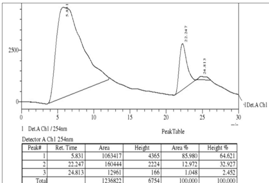
Fig 2: HPLC analysis of pesticide polluted soil sample of kattamannarkoil
