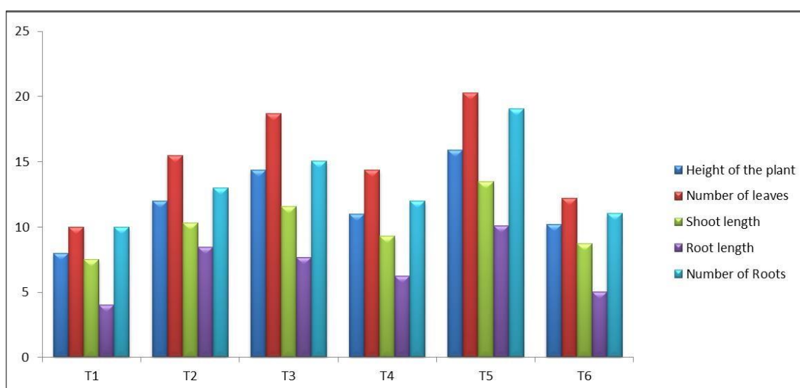
Fig 1: Effect of fertilizers on Height and Number of leaves in Lycopersicum esculentum (45 th day)
