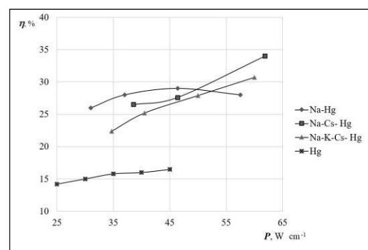
Fig 2: Dependence of light efficiency (η) on the lamps specific power (P l ) with various filling of a digit tube: Na-Hg (HPS 400); Na-Cs-Hg (HPS-Cs 400), Na-K-Cs-Hg (HPS-Cs-K 400)
