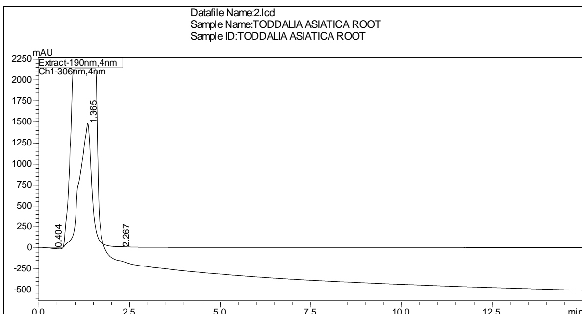
Fig 2: HPLC analysis of root extract of Toddalia asiatica
