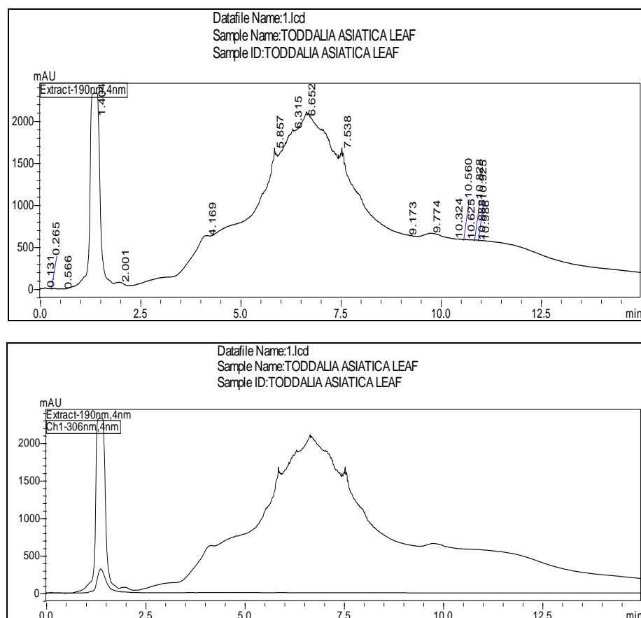
Fig 1: HPLC analysis of leaf extract of Toddalia asiatica
