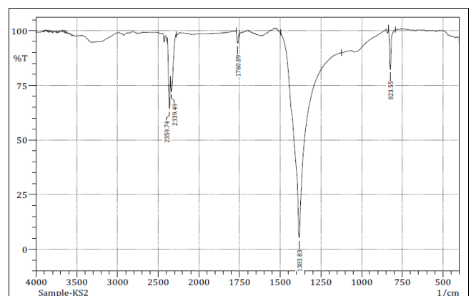
Fig 3: FTIR spectrum analysis of silver nanoparticles using Hypnea valentiae (Turner) Montagne
