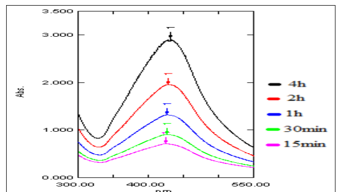
Fig 2: UV-Visible spectrum of silver nanoparticles using Hypnea valentiae (Turner) Montagne
