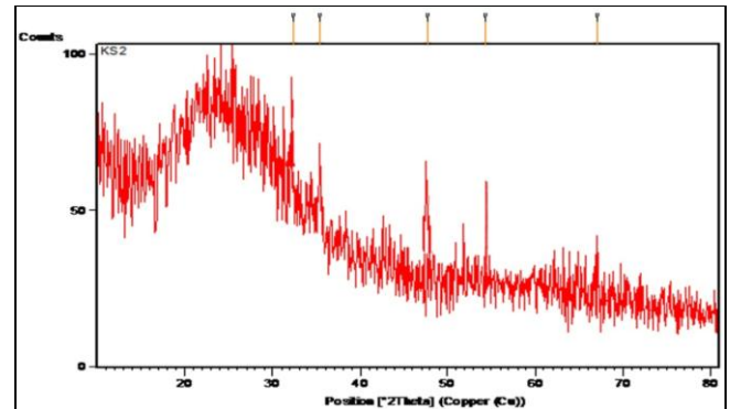
Fig 4: XRD spectrum analysis of silver nanoparticles using Hypnea valentiae (Turner) Montagne
